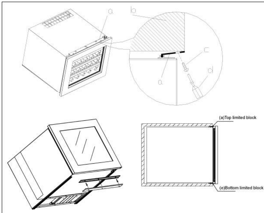
a. Top limited block b. Kitchen cabinet c. Screw d. Screwdriver e. Bottom limited block
